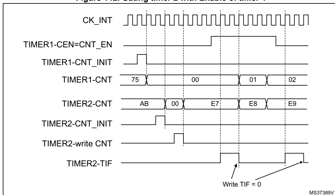
Figure 142. Gating timer 2 with Enable of timer 1
